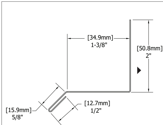
No. M50H.A Drip flashing
