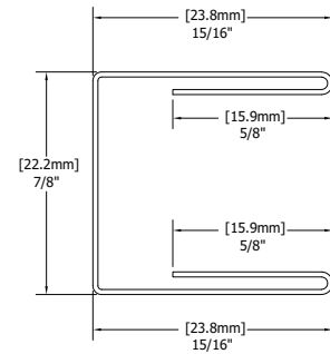
No. M06H (BB & RBB) Batten trim filler
